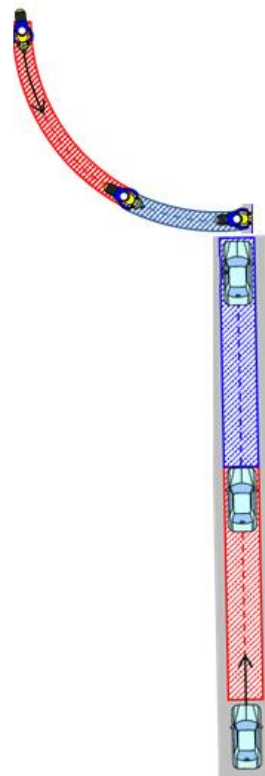
Figure 2.10: Methods of calculating collision risk – Enhanced "Ghost Vehicles" with PTW curvature
