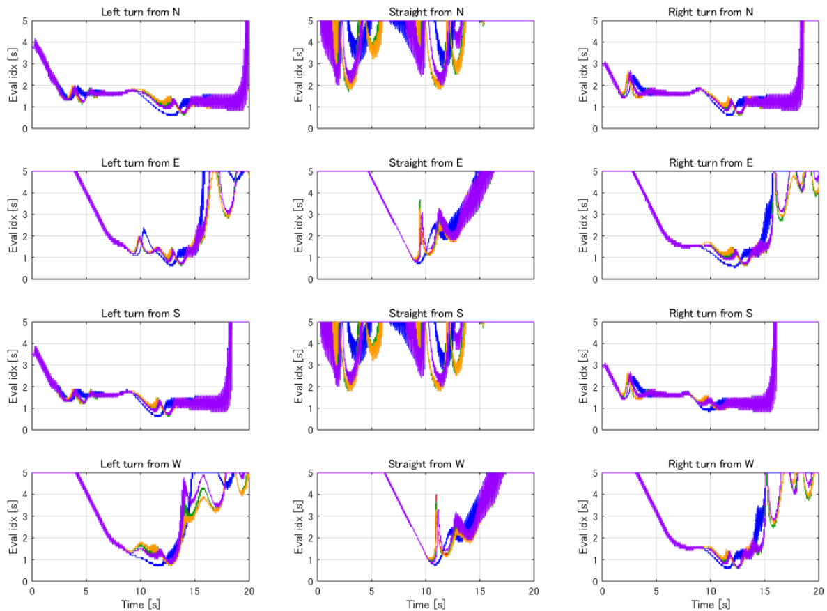
Figure 3.17: Evaluation indexes with 1.0[Hz] filter (All patterns)
