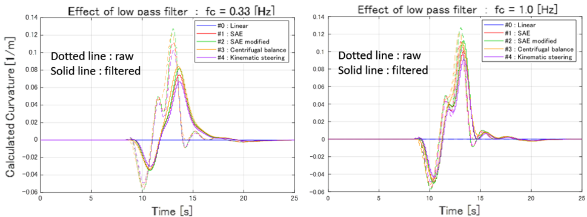
Figure 3.6: Effect of low pass filter (Left turn from E)
