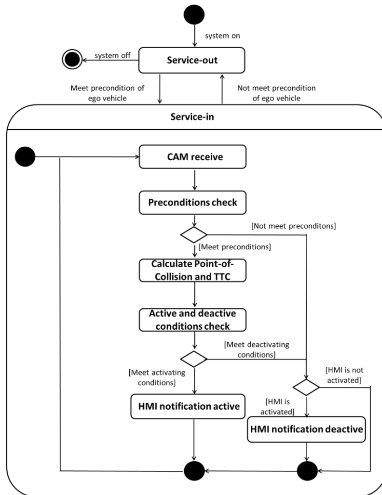
Figure 2.12: Flowchart of receiving CAM - Level B
