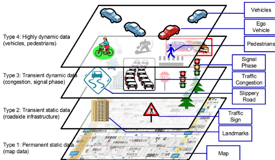
Figure 6.2: Four types of the LDM [22; p. 103]
